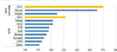
Figure 4: Highest pack-level energy density of commercially deployed NCM & Semi-Solid-State battery packs for PV
